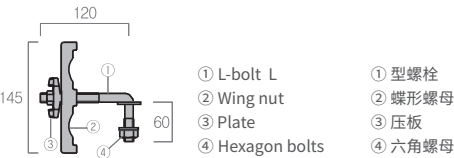
P50-F3BA 50*50 Steel pipe fixing bolt components50*50 钢管固定螺栓组件
