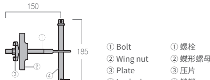
BFP8-F4A Keel fixing bolt components 龙骨固定螺栓组件
