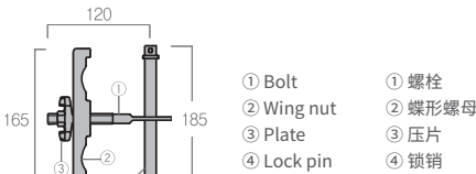
P50-F4A 50*50 Steel pipe fixing bolt components50*50 钢管固定螺栓组件
