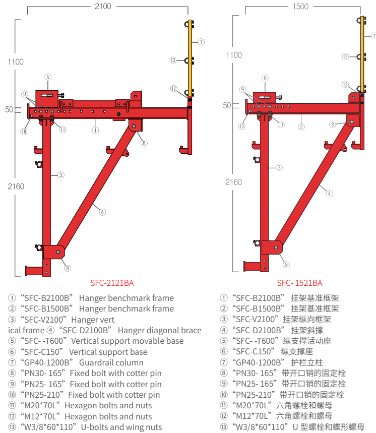
Single-side formwork hanging bracket 单侧模板挂架
