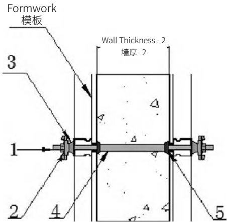
Sleeve-type Tie Bolt 套管式对拉螺栓
